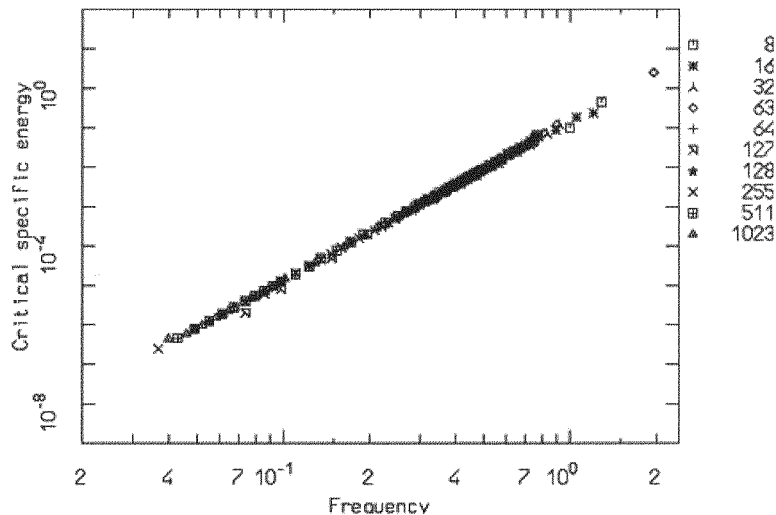
Fig. 2. Plot of the numerically calculated values of E^R(N, \omega) vs. \omega , for different values of N as identified by the different symbols but with the specific energy \varepsilon = E/N in ordinates. All the data look well aligned on the same curve (possibly a straight line). This defines the function \varepsilon_c(\omega) , as stated in the text.
