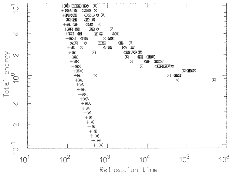
Fig. 1. Relaxation time t_s^R for varying energy and number of modes in a packet. Moving horizontally, i.e., at a fixed energy, the packet of the first s modes loses 20% if its initial energy at time t_s^R . At a given energy, only a small packet of modes takes part on the sharing on energy in a short time. Different symbols correspond to different values of s = 1, 2, \dots , from left to right. This figure is drawn for N = 16 .
