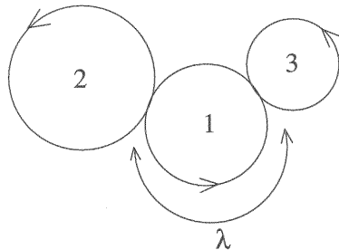
Fig. 2. A circle cactus with 3 circles
