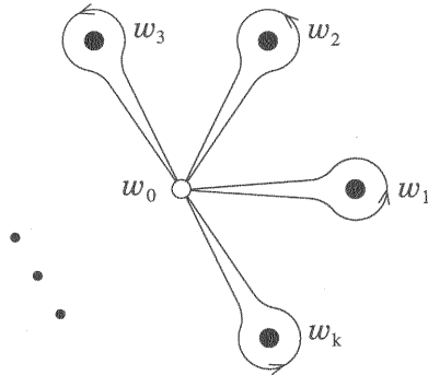
Fig. 1. A star of loops
