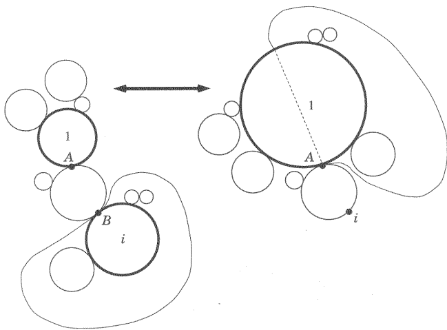
Fig. 3. Merging two circles
