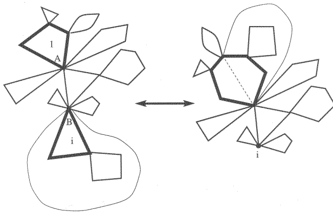
Fig. 5. Merging two polygons
