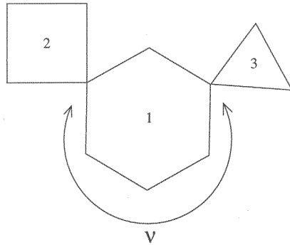
Fig. 4. A cactus composed of 3 polygons
