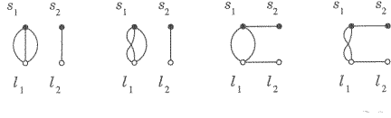
Fig. 7. The four graphs that contribute to the term \frac{2}{3} l_1^2 s_1^2
