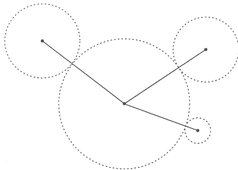
Fig. 6. Replacing a constellation by its dual
