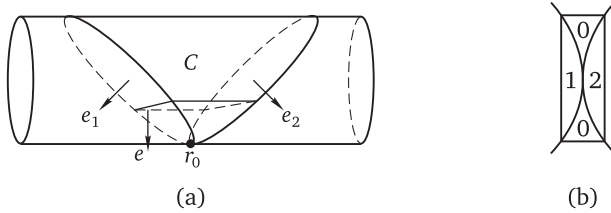
FIG. 4. (a) C is the part of a cylinder bounded by two planes through r_0 ; (b) the projections of S_t^1 , S_t^2 , and S_t^0 on the xy -plane are marked by «1», «2», and «0», respectively
