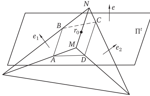
FIG. 3. r_0 lies on the edge MN of the tetrahedron, and the section of the tetrahedron by the plane \Pi^t: (r - r_0, e) = -t is the quadrilateral ABCD
