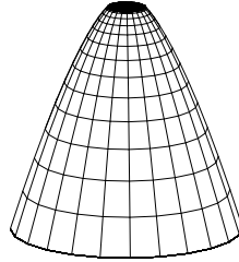
FIG. 1. The solution of Newton's problem with M = 2
