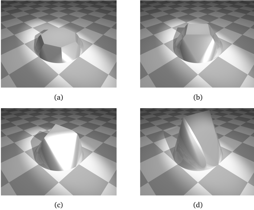
FIG. 2. Numerical solutions of Problem 1 in the cases (a) M = 0.4 ; (b) M = 0.7 ; (c) M = 1.0 ; (d) M = 1.5
