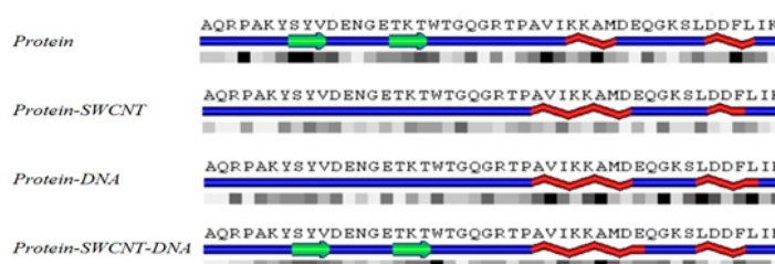
FIG. 4. The secondary structure of the H-NS, along with the solvent accessible surface area for its residues.
