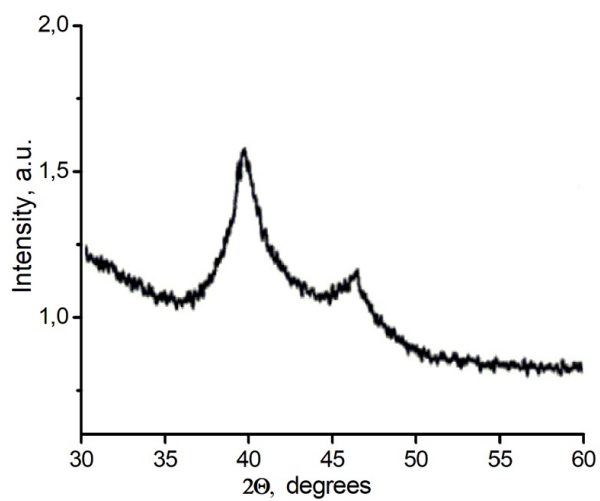
FIG. 1. XRD patterns of Pt-NPs/RGO composite
